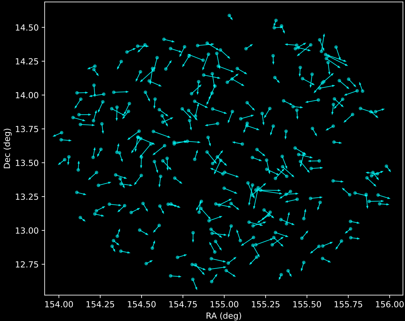
GALAH DR4 Noise Stream Proper Motion Vectors (n=257)
