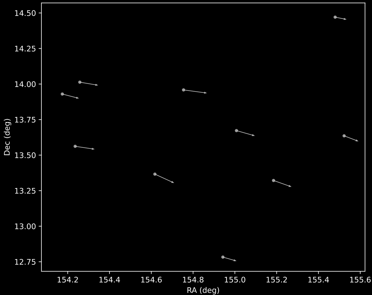
GALAH DR4 Cluster 15 Proper Motion Vectors (n=10)
