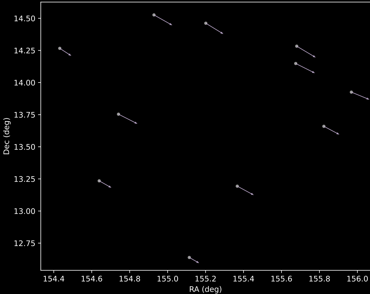
GALAH DR4 Cluster 9 Proper Motion Vectors (n=11)
