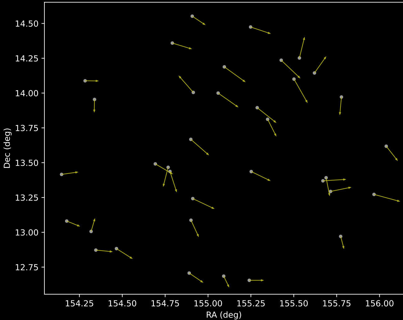
GALAH DR4 Cluster 16 Proper Motion Vectors (n=36)
