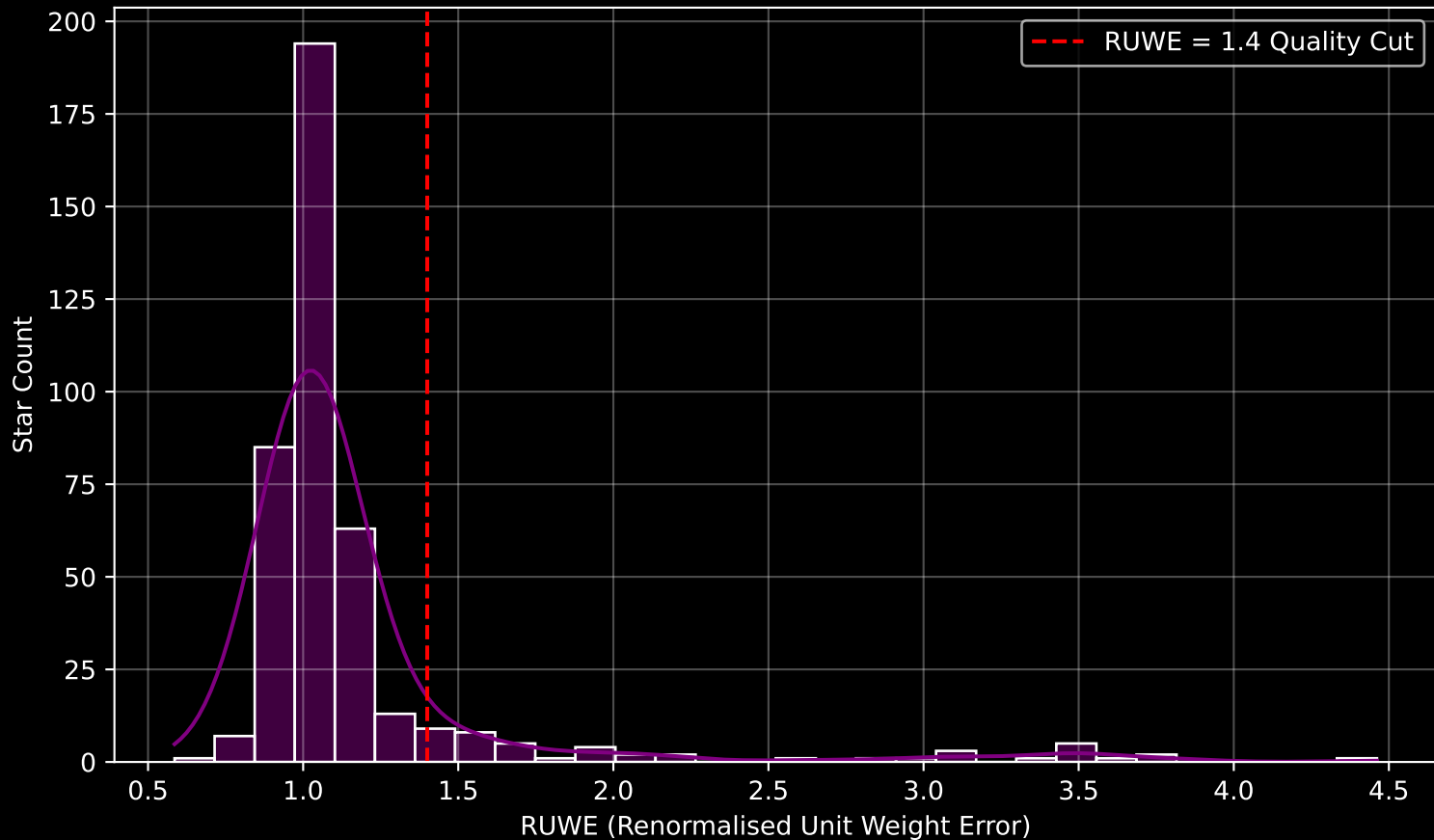
GALAH DR4 Field [6600] RUWE Distribution (n= 410)
