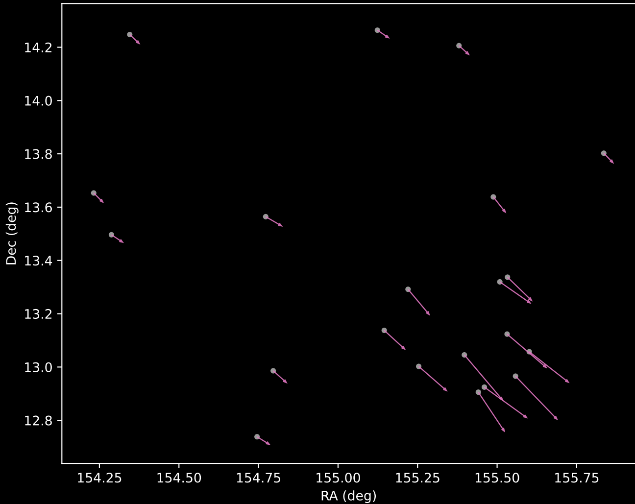
GALAH DR4 Cluster 12 Proper Motion Vectors (n=21)
