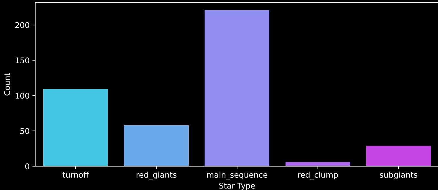
GALAH DR4 Field: [6600] Count plot of Star Type
